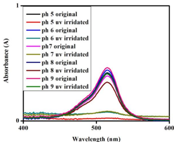
Fig. 14: Effect of pH on the degradation of dye using \text{SnO}_2 nanoparticles under UV light.
