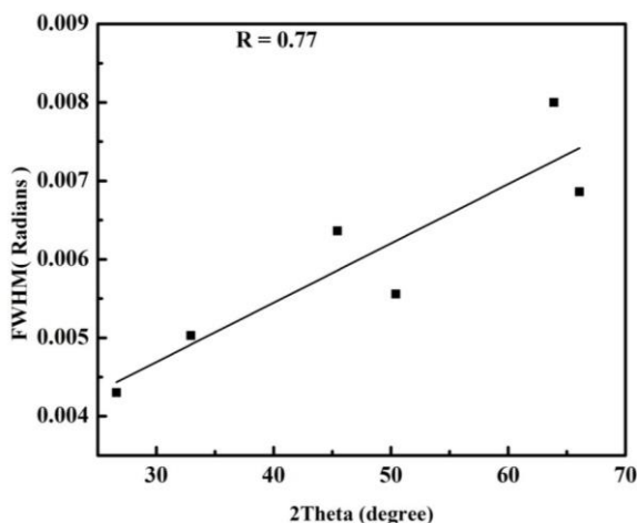
Fig. 7: Two Theta Vs FWHM curve of \text{SnO}_2 nanoparticles.
