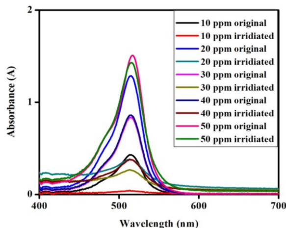
Fig. 13: Effect of initial concentration on the degradation of dye using \text{SnO}_2 nanoparticles under UV light.
