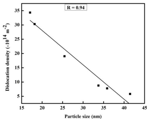
Fig. 2: Particle size Vs dislocation density curve of SnO 2 nanoparticles
